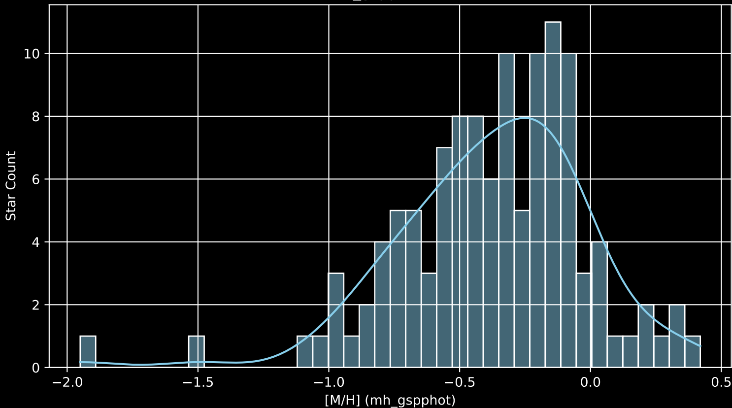
GALAH DR4 Field: [7245] [M/H] (mh_gspphot) (n= 117)
