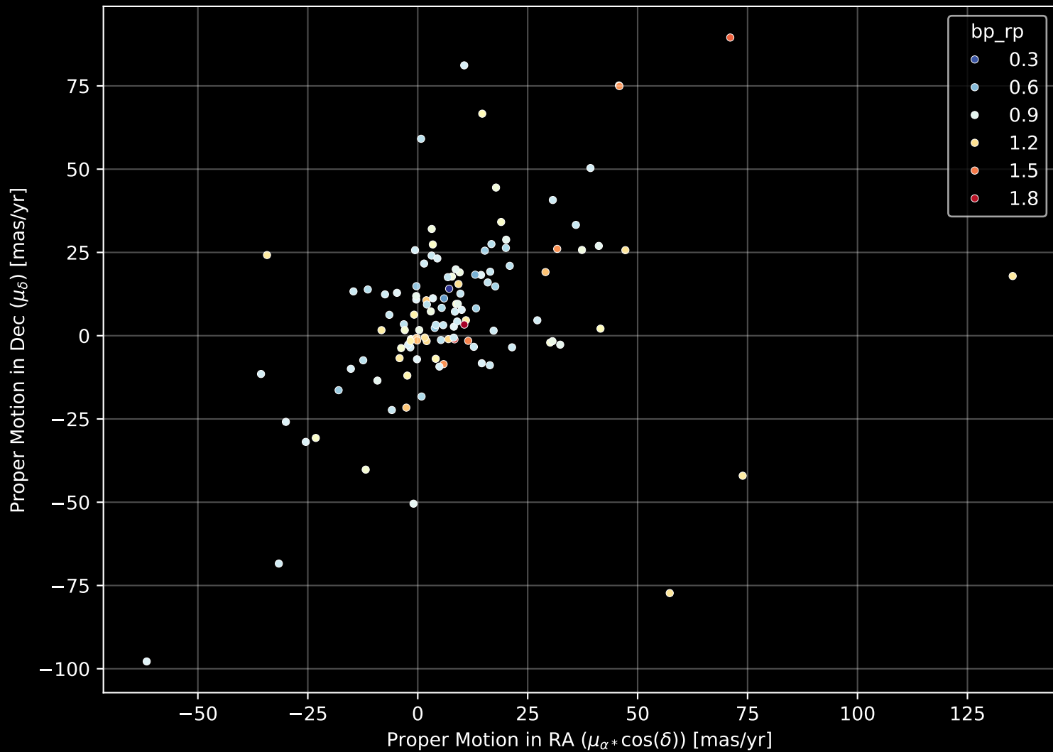
GALAH DR4 Field: [7245] Proper Motion Diagram (n= 119)
