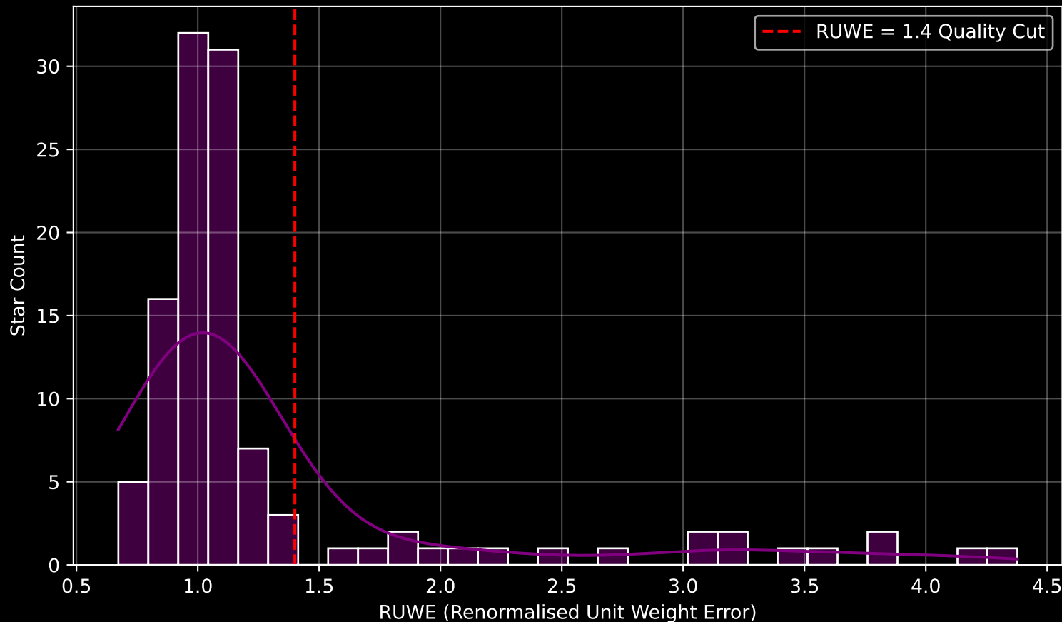
GALAH DR4 Field [7245] RUWE Distribution (n= 113)
