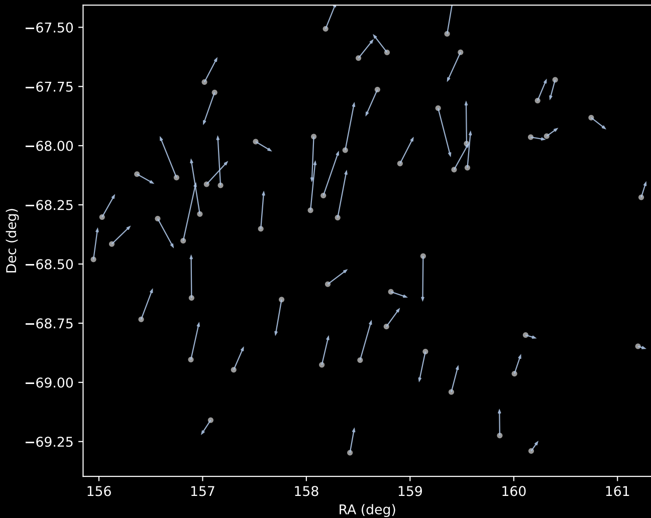
GALAH DR4 Cluster 1 Proper Motion Vectors (n=56)
