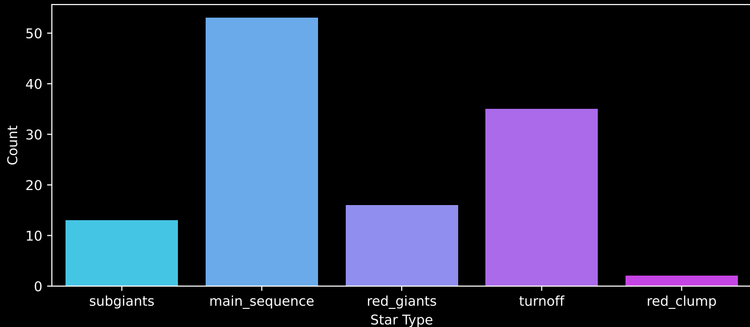
GALAH DR4 Field: [7245] Count plot of Star Type
