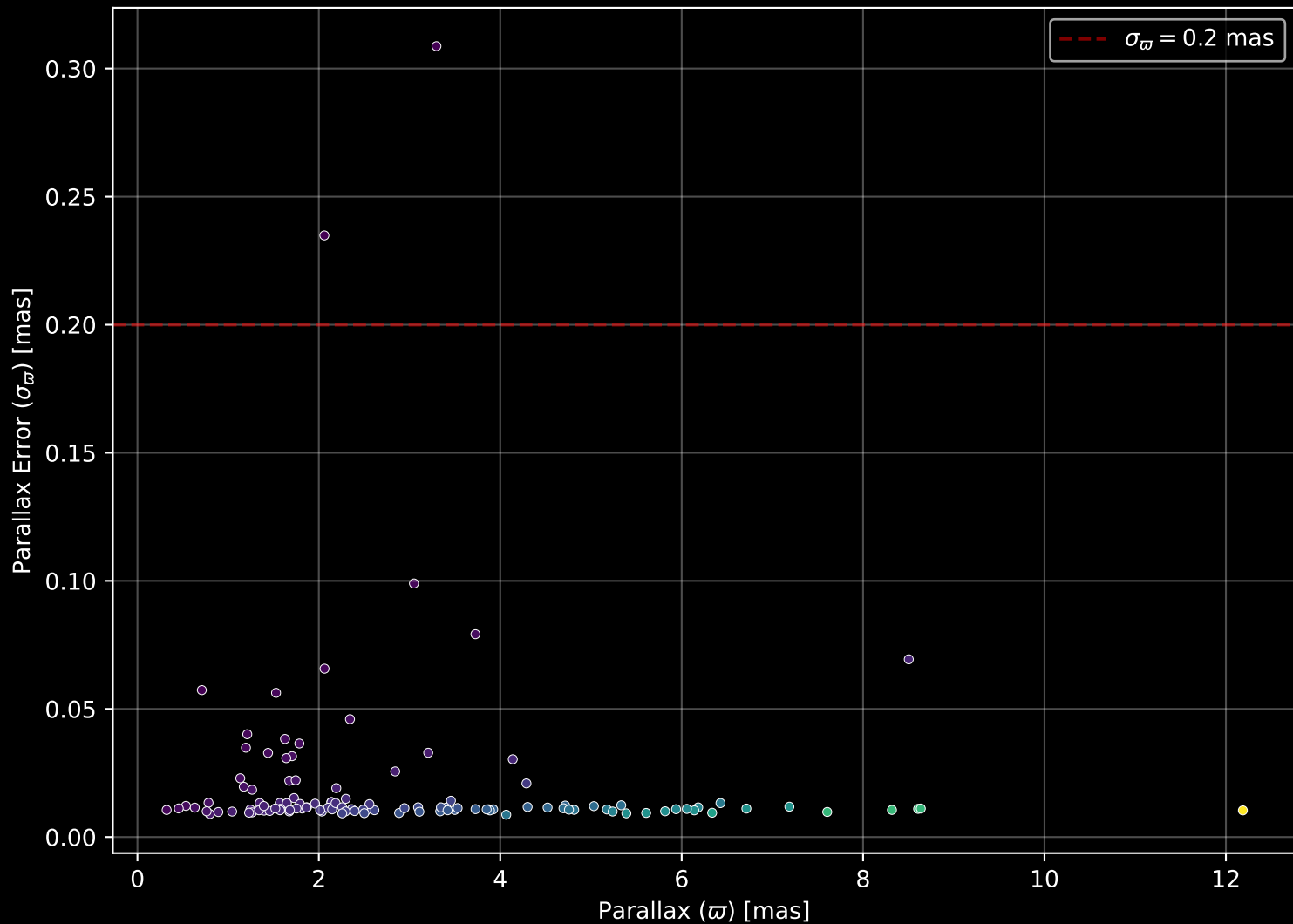
GALAH DR4 Field: [7245] Parallax Quality (n= 119)
